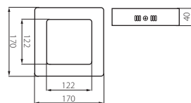
KANTI LED SMD 13W-NW
