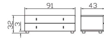
2 Schubladen/2 tiroirs/2 drawers
