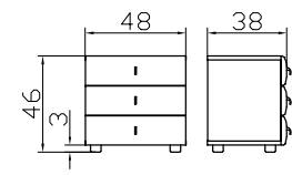
3 Schubladen/3 tiroirs/3 drawers
