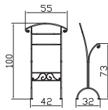
Bruce Herrendiener/ valet /dressboy Massiveisen handgeschmiedet Fer forgé à la main Solid iron handforged
